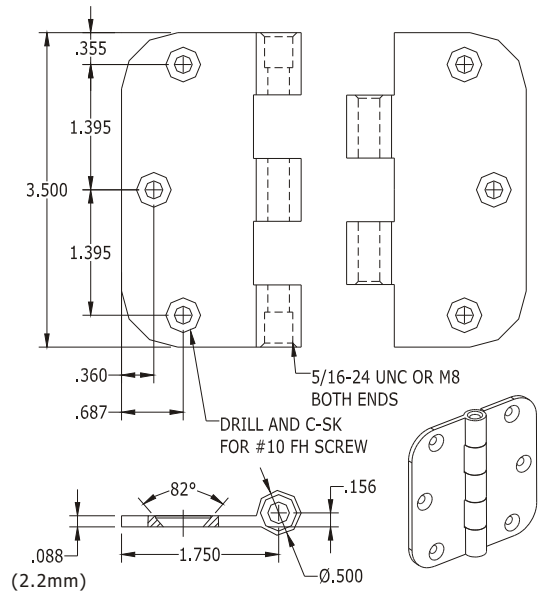
3.5×3.5×.088 (2.2mm) INCH RADIUS CORNER HINGE WEIGHT: 0.445LB (202g)
