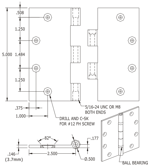
5×5×.146 (3.7mm) INCH SQ HINGE WITH BALL BEARING WEIGHT: 1.239LB (562g)
