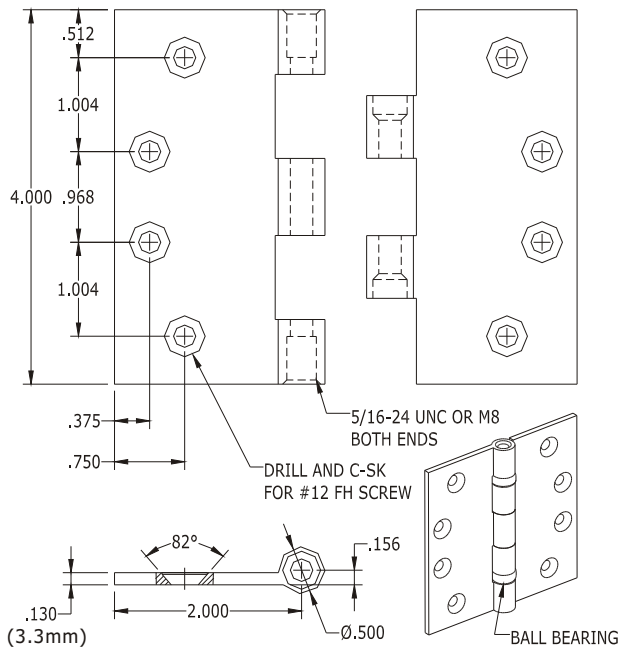
4×4×.130 (3.3mm) INCH SQ HINGE WITH BALL BEARING WEIGHT: 0.766LB (347g)
