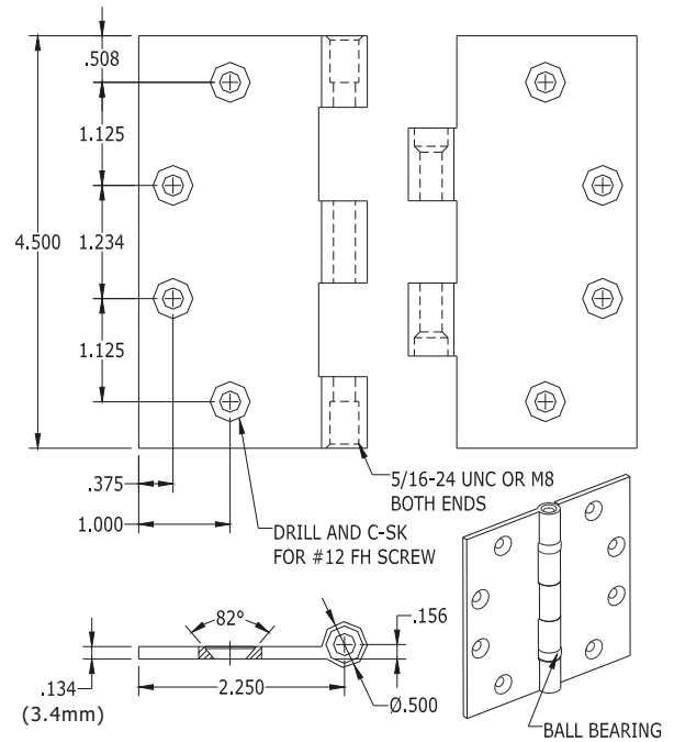
4.5×4.5×.134 (3.4mm) INCH SQ HINGE WITH BALL BEARING WEIGHT: 0.957LB (434g)
